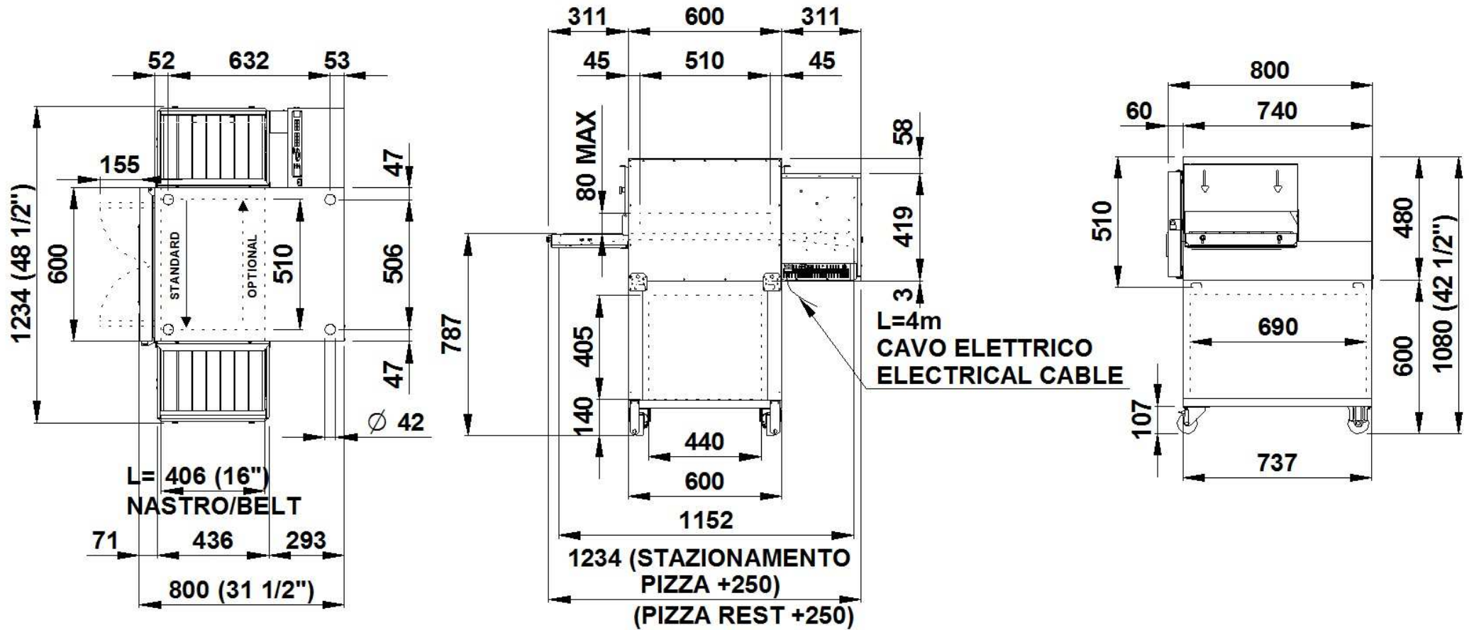
TOP VIEW
